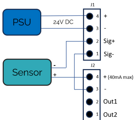
2-Wire Interface
